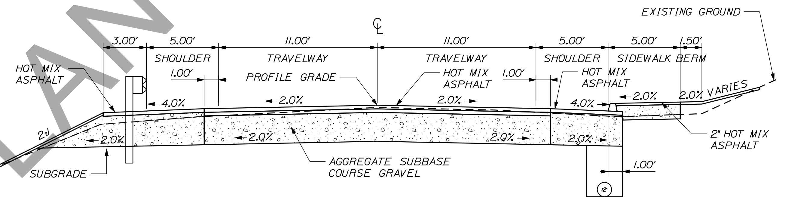
FULL CONSTRUCTION GUARDRAIL LEFT
