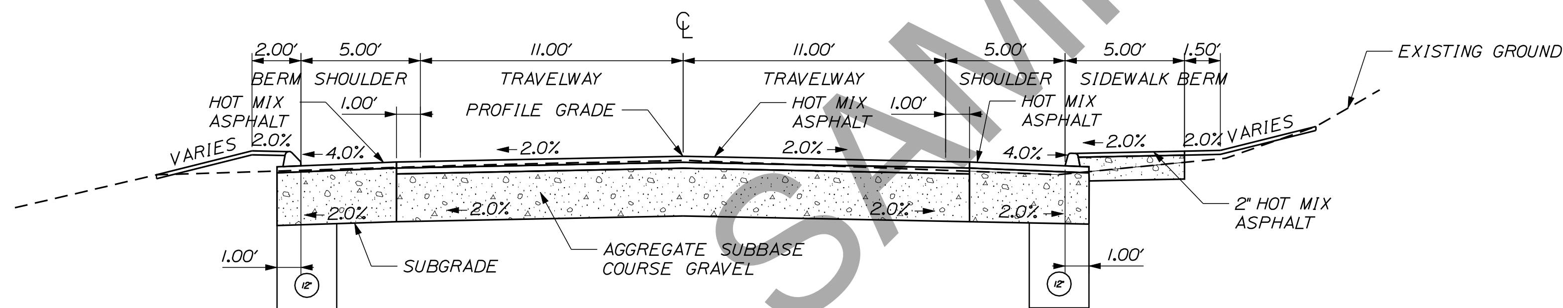
FULL CONSTRUCTION W/SIDEWALK
